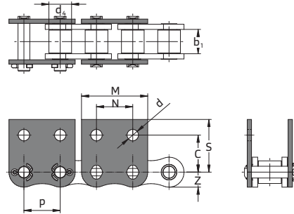
extended link plate on both sides WSK-2
