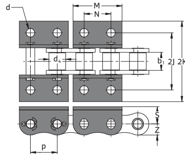
bent plates with angle on both sides WK-2
