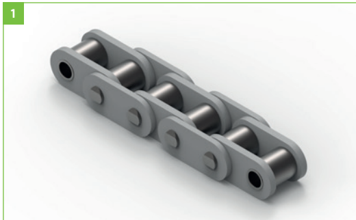
Figure 1: Roller chain with straight link plates
