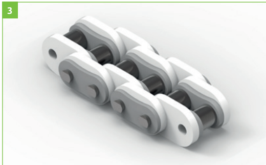
Figure 3: Roller chain with plastic link plates
