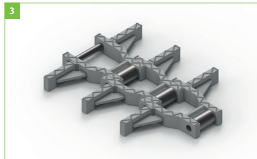
Figure 3: "Reinforced clinker" series WHX HD
