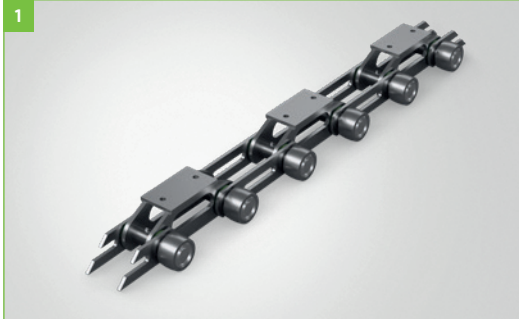
Figure 1: Oil-tight reclaimer chain with SCS PO
