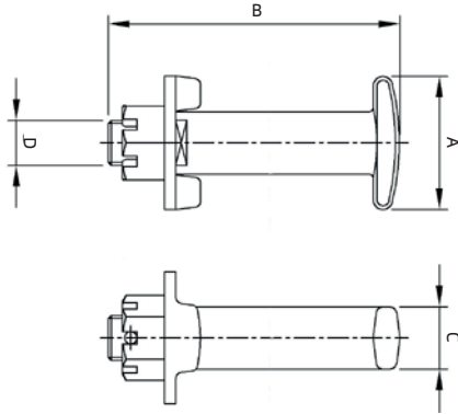
T-pin with thread + washer + castle nut
